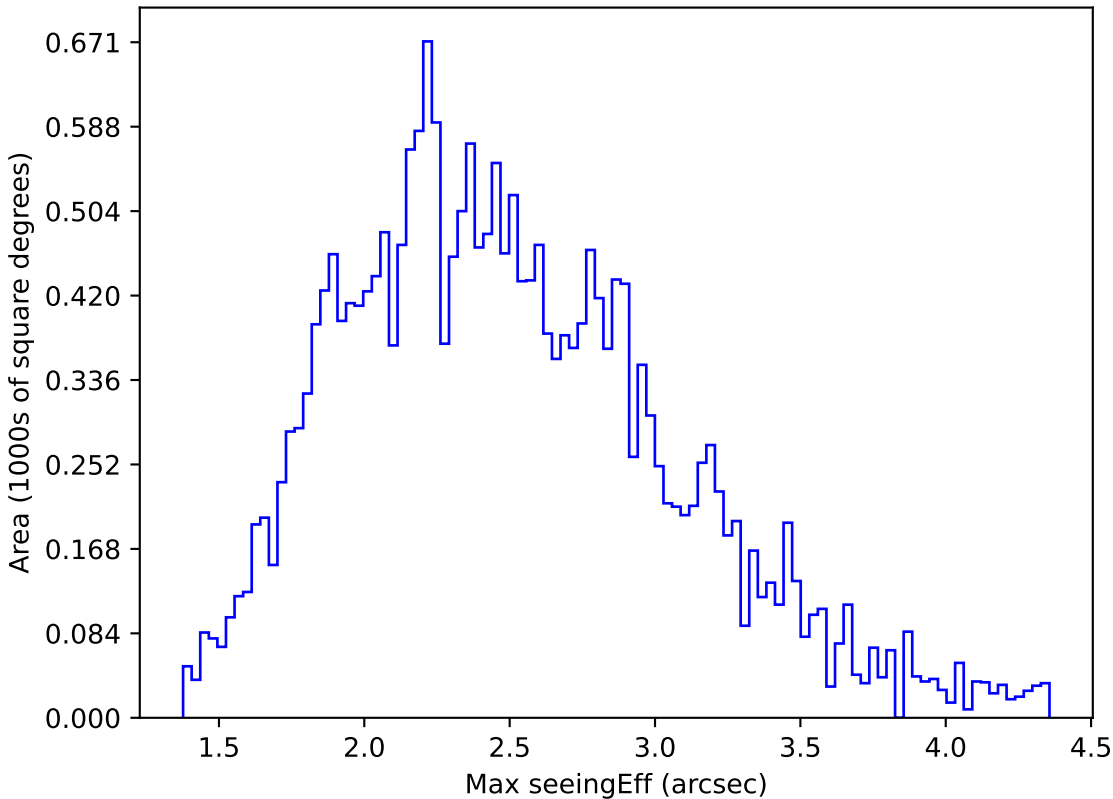
too_elab_r64_d3_giz_v3.4_10yrs All sky u band: Max seeingEff
