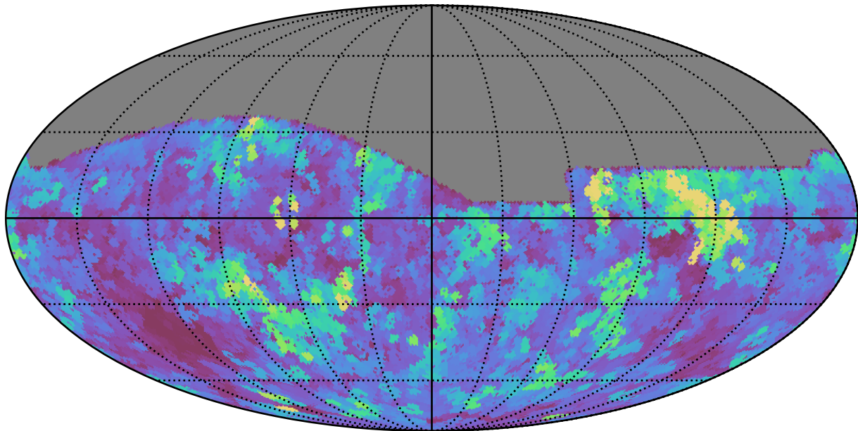
too_elab_r64_d3_giz_v3.4_10yrs All sky g band: Max seeingEff
