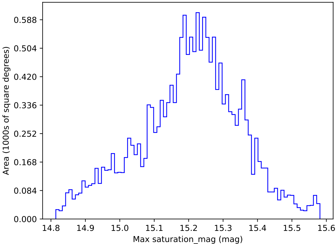
too_elab_r64_d3_giz_v3.4_10yrs WFD z band: Max saturation_mag
