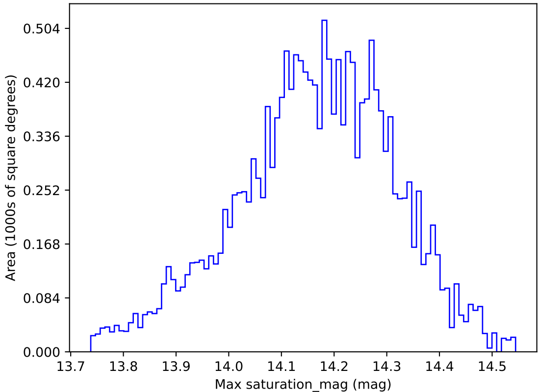
too_elab_r64_d3_giz_v3.4_10yrs WFD y band: Max saturation_mag
