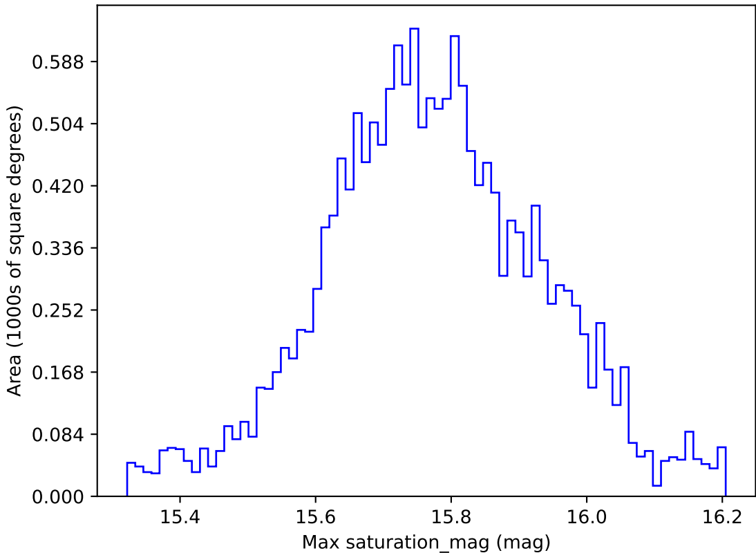
too_elab_r64_d3_giz_v3.4_10yrs WFD r band: Max saturation_mag
