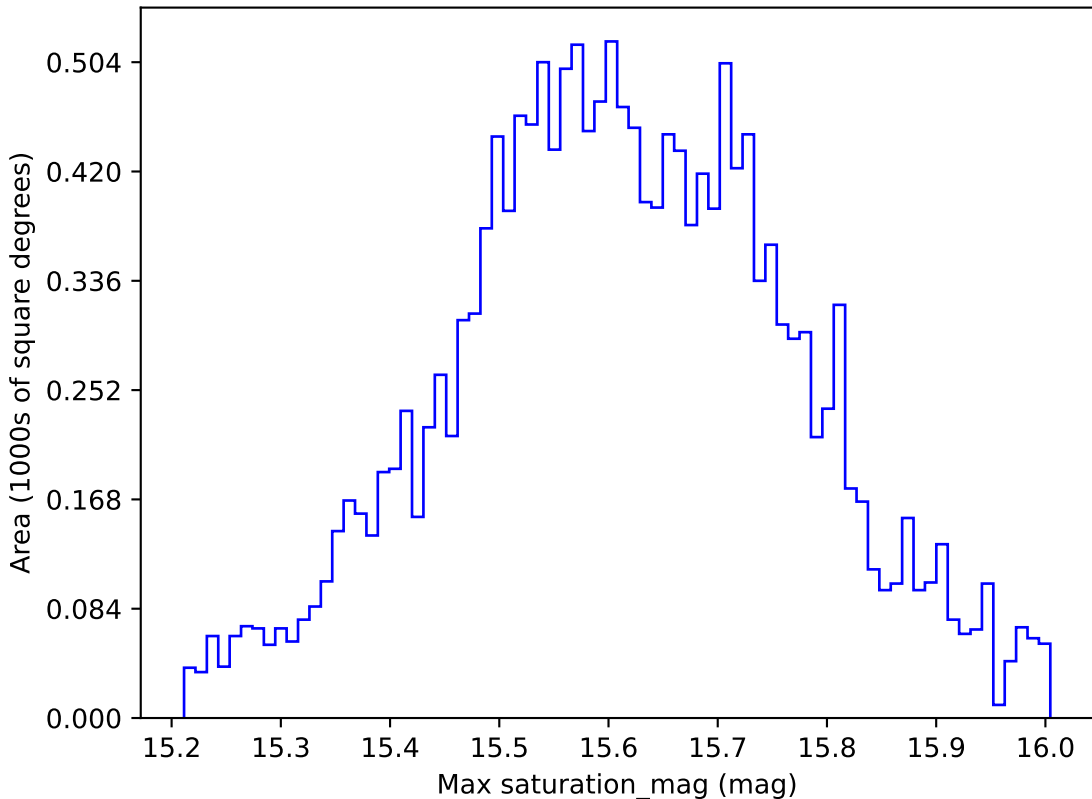
too_elab_r64_d3_giz_v3.4_10yrs WFD i band: Max saturation_mag
