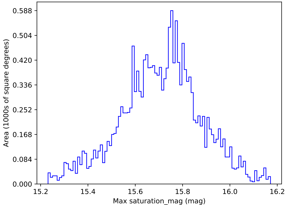
too_elab_r64_d3_giz_v3.4_10yrs WFD g band: Max saturation_mag
