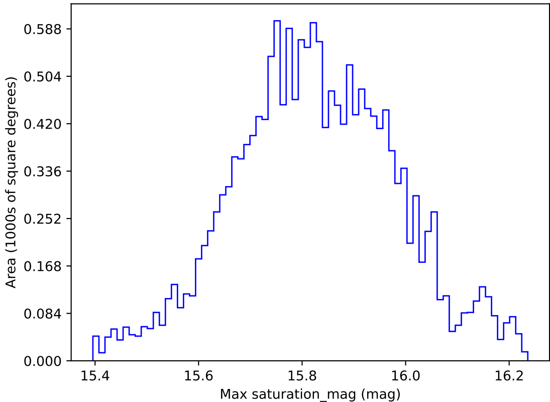
too_elab_r64_d3_giz_v3.4_10yrs WFD all bands: Max saturation_mag
