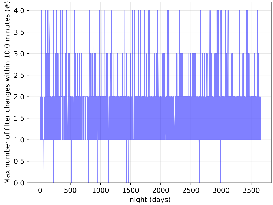
too_elab_r64_d3_giz_v3.4_10yrs Per Night: Max number of filter changes within 10.0 minutes
