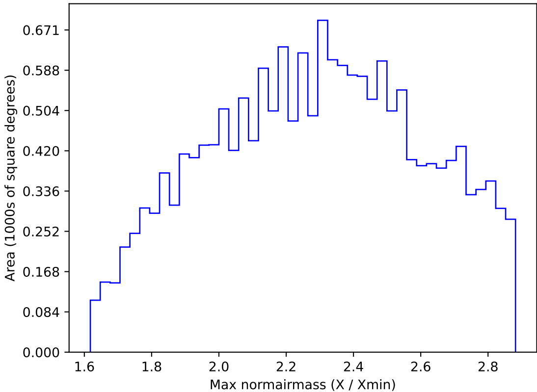
too_elab_r64_d3_giz_v3.4_10yrs WFD z band: Max normairmass
