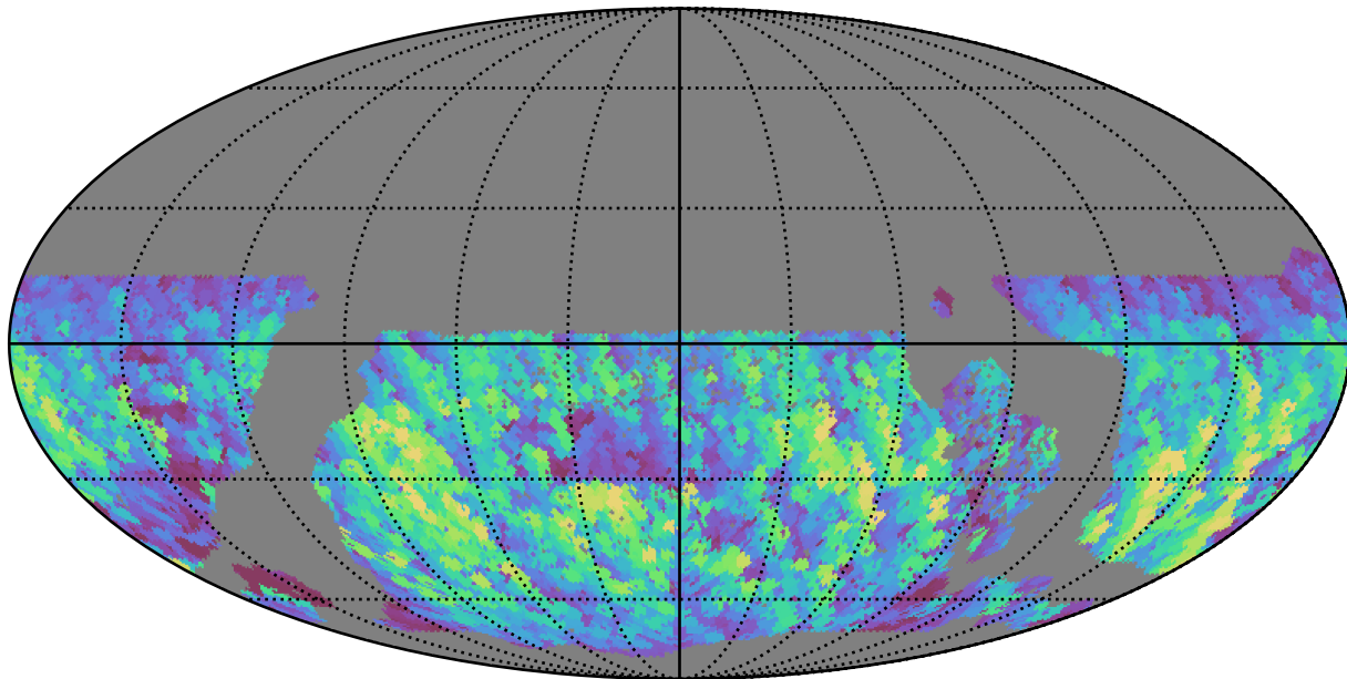
too_elab_r64_d3_giz_v3.4_10yrs WFD y band: Max normairmass
