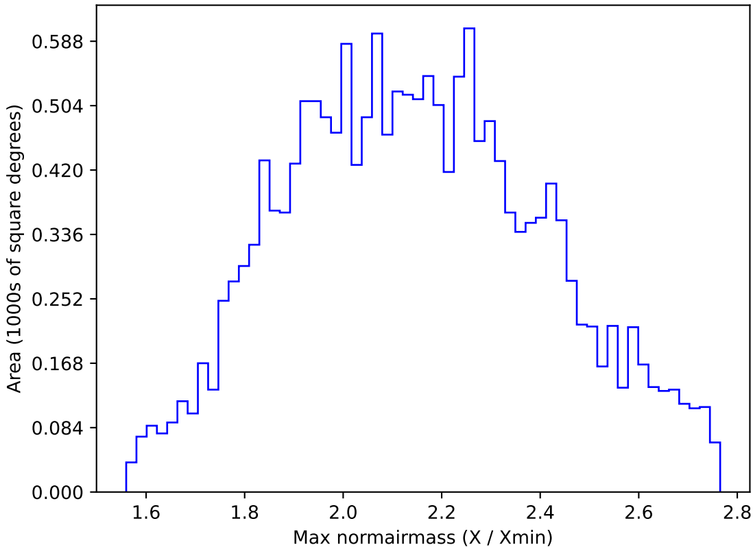
too_elab_r64_d3_giz_v3.4_10yrs WFD y band: Max normairmass
