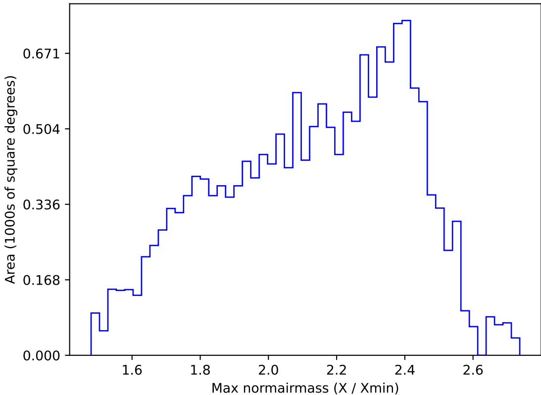
too_elab_r64_d3_giz_v3.4_10yrs WFD r band: Max normairmass
