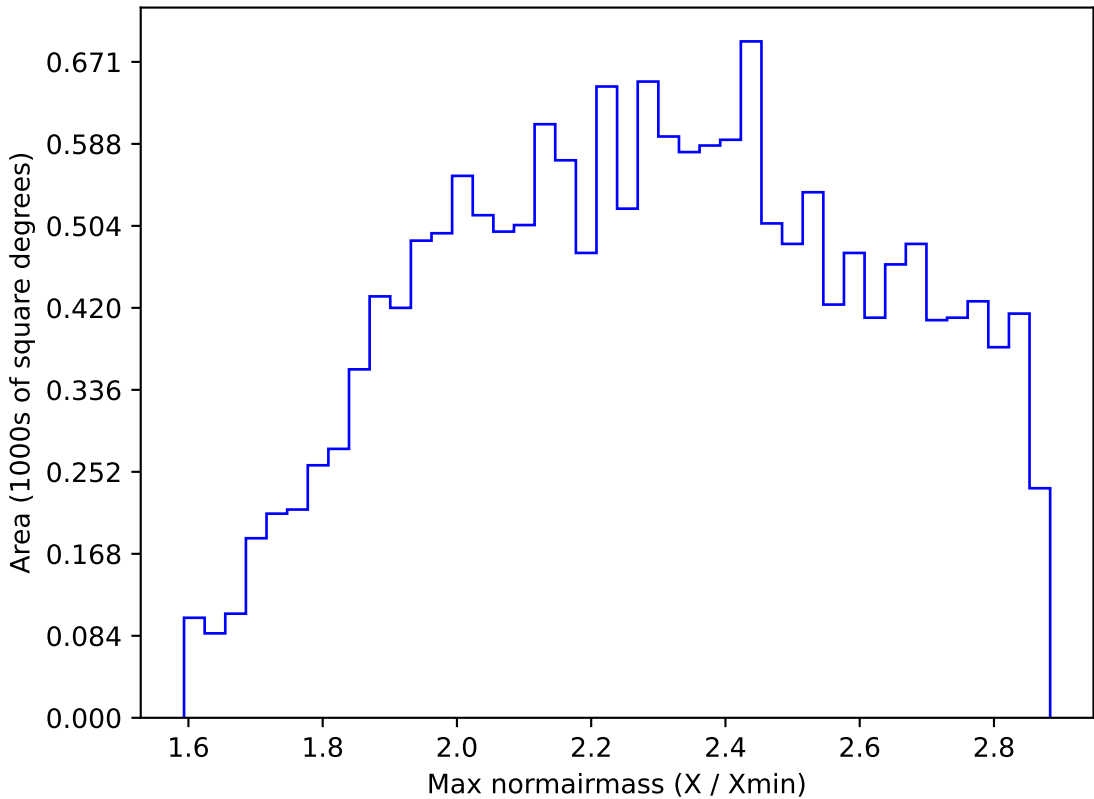
too_elab_r64_d3_giz_v3.4_10yrs WFD i band: Max normairmass
