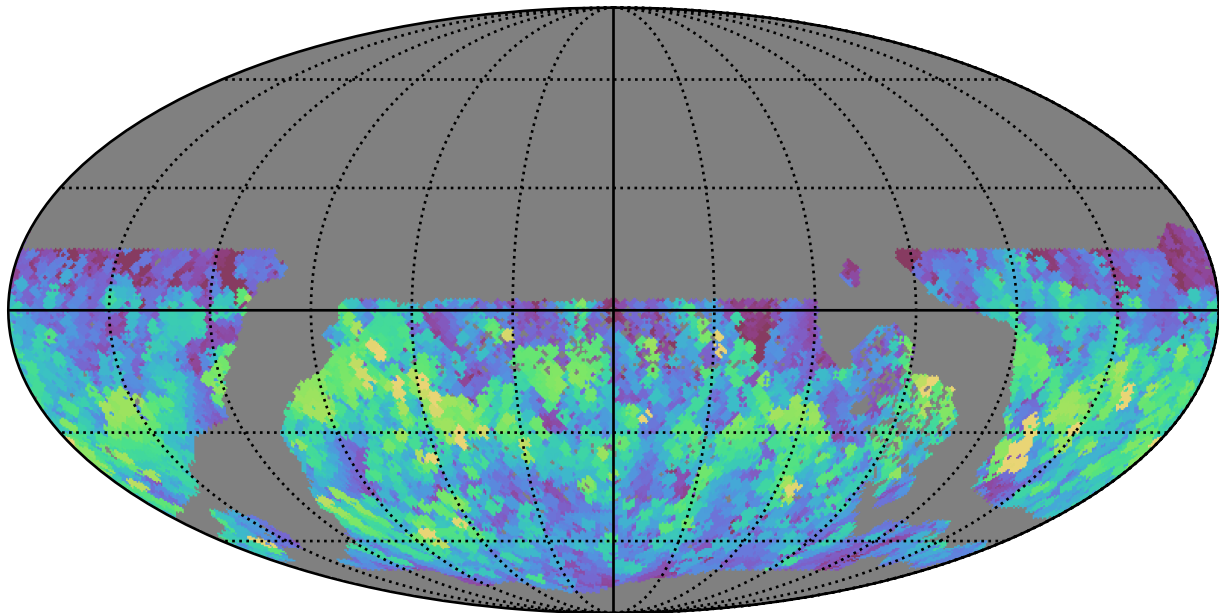
too_elab_r64_d3_giz_v3.4_10yrs WFD g band: Max normairmass
