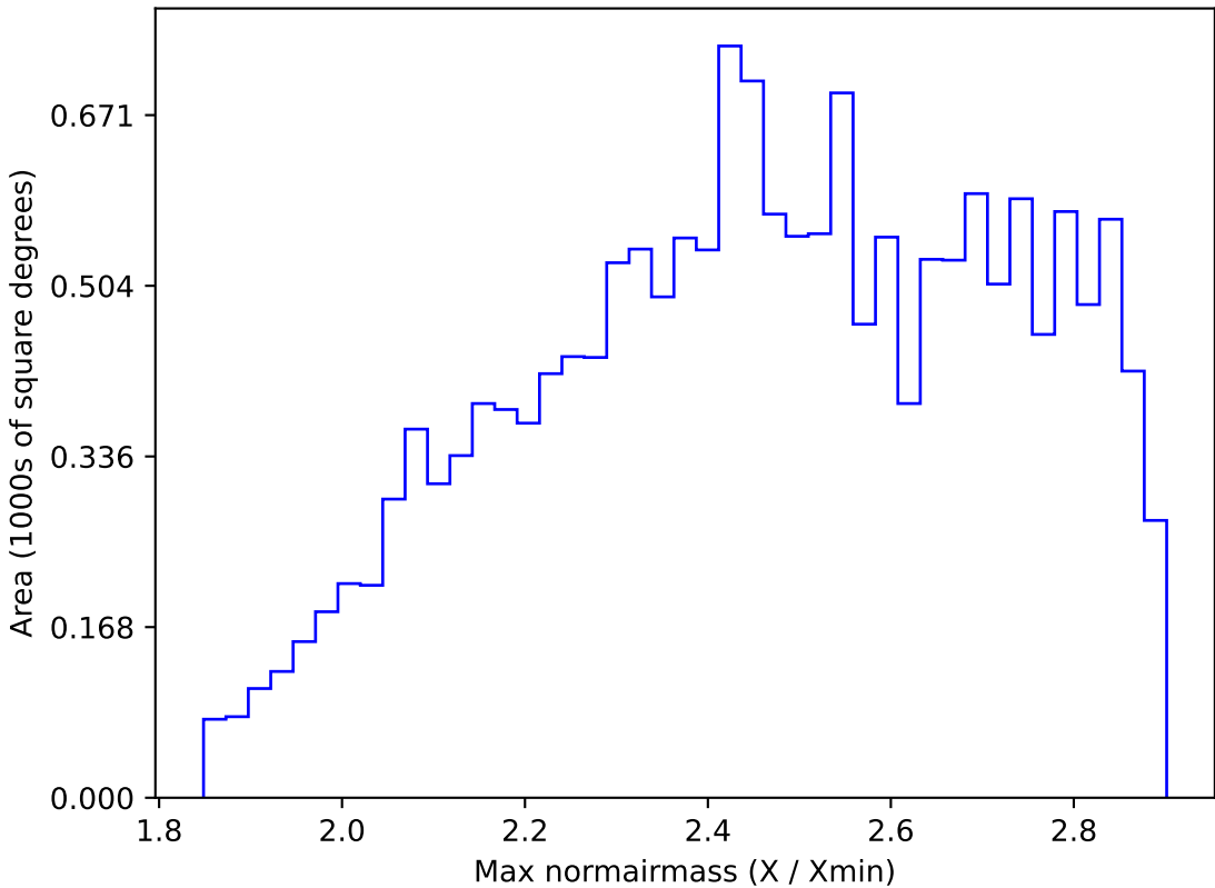
too_elab_r64_d3_giz_v3.4_10yrs WFD all bands: Max normairmass
