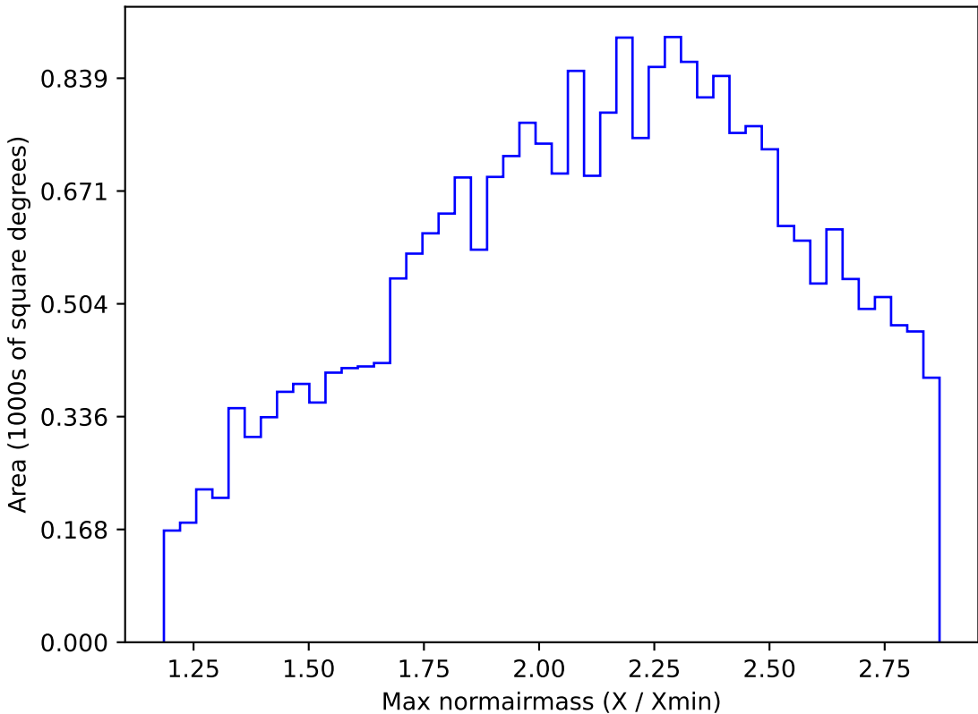
too_elab_r64_d3_giz_v3.4_10yrs All sky z band: Max normairmass
