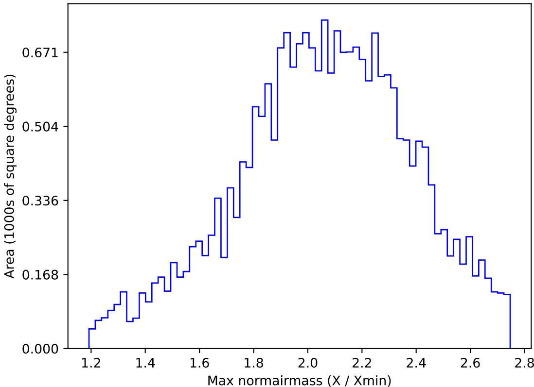
too_elab_r64_d3_giz_v3.4_10yrs All sky y band: Max normairmass
