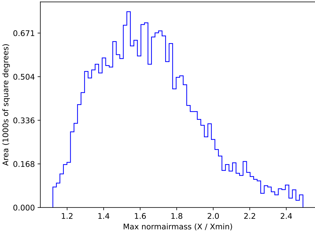
too_elab_r64_d3_giz_v3.4_10yrs All sky u band: Max normairmass
