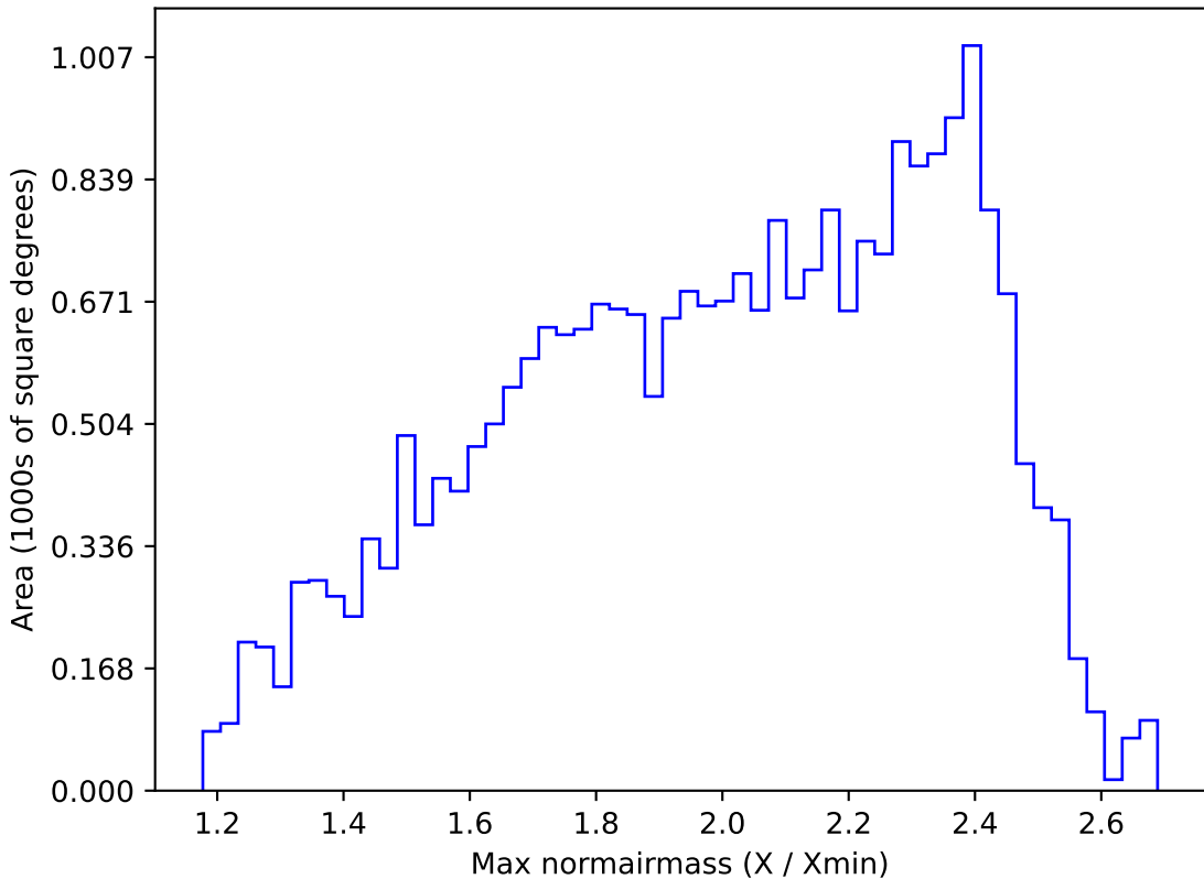
too_elab_r64_d3_giz_v3.4_10yrs All sky r band: Max normairmass
