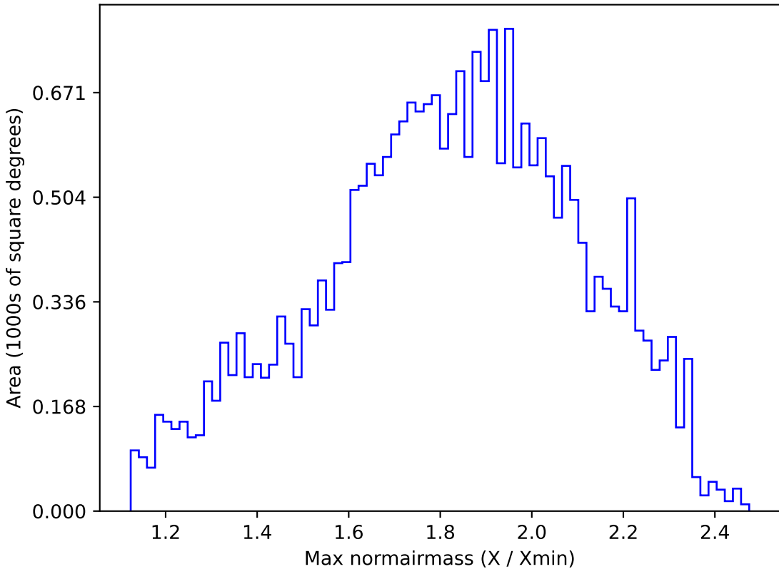
too_elab_r64_d3_giz_v3.4_10yrs All sky g band: Max normairmass
