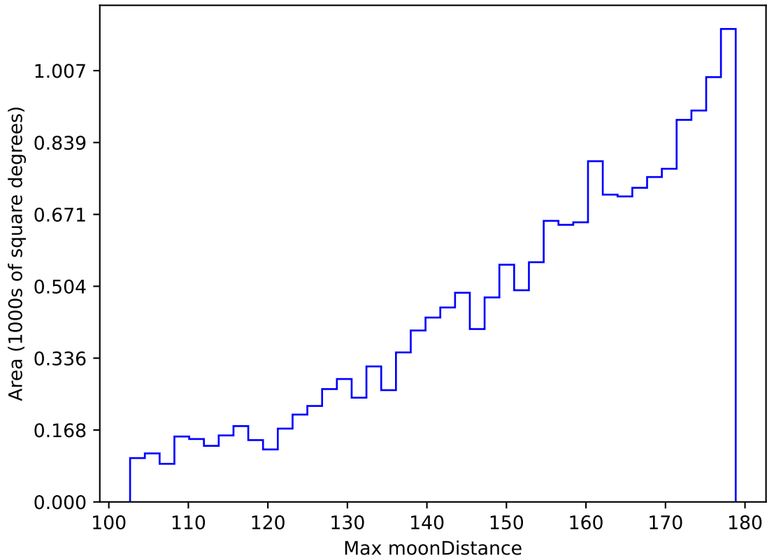
too_elab_r64_d3_giz_v3.4_10yrs WFD z band: Max moonDistance
