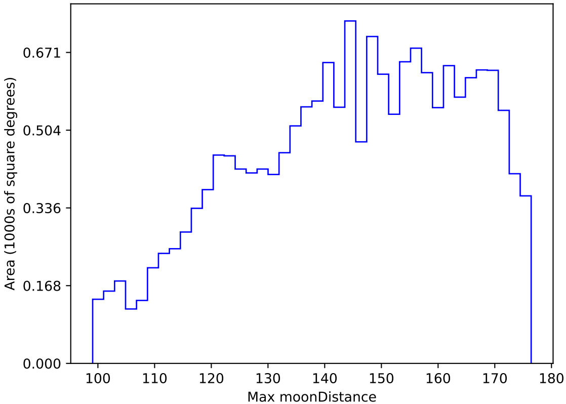
too_elab_r64_d3_giz_v3.4_10yrs WFD y band: Max moonDistance
