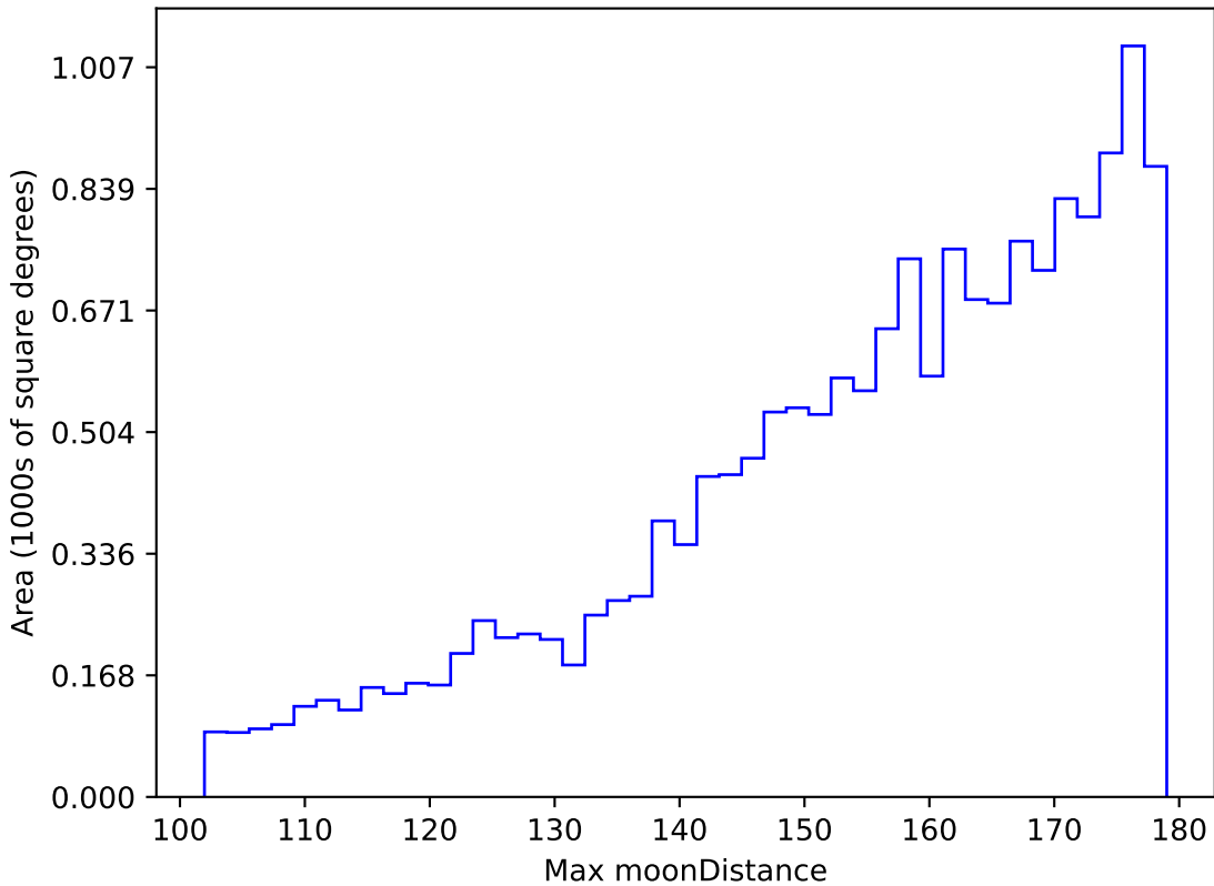
too_elab_r64_d3_giz_v3.4_10yrs WFD u band: Max moonDistance
