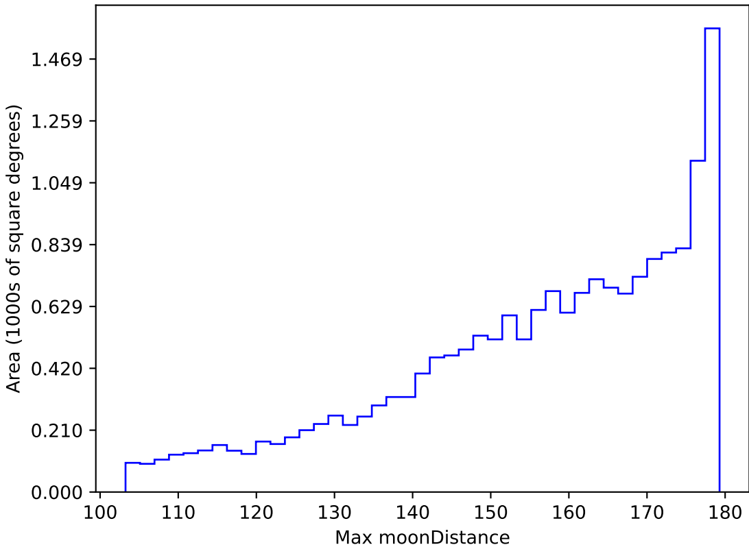
too_elab_r64_d3_giz_v3.4_10yrs WFD r band: Max moonDistance
