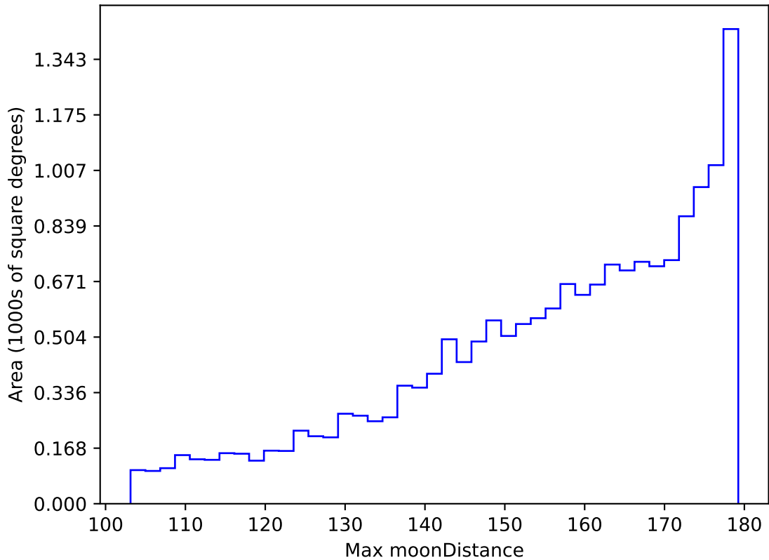
too_elab_r64_d3_giz_v3.4_10yrs WFD i band: Max moonDistance
