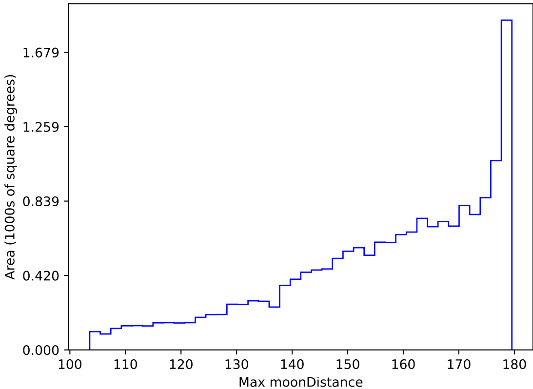
too_elab_r64_d3_giz_v3.4_10yrs WFD all bands: Max moonDistance
