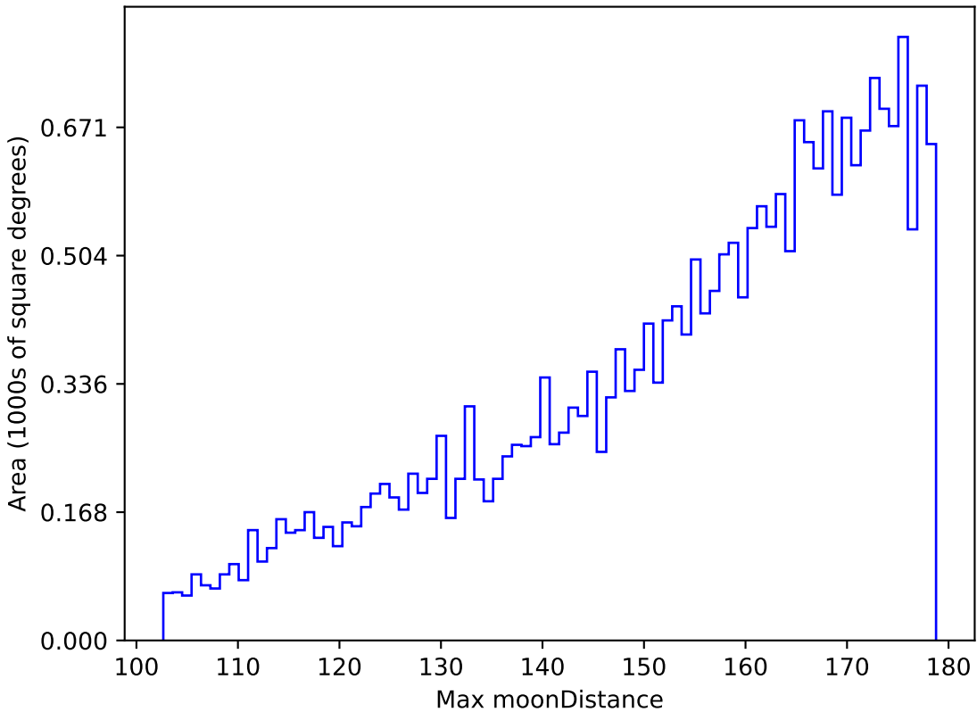
too_elab_r64_d3_giz_v3.4_10yrs All sky z band: Max moonDistance
