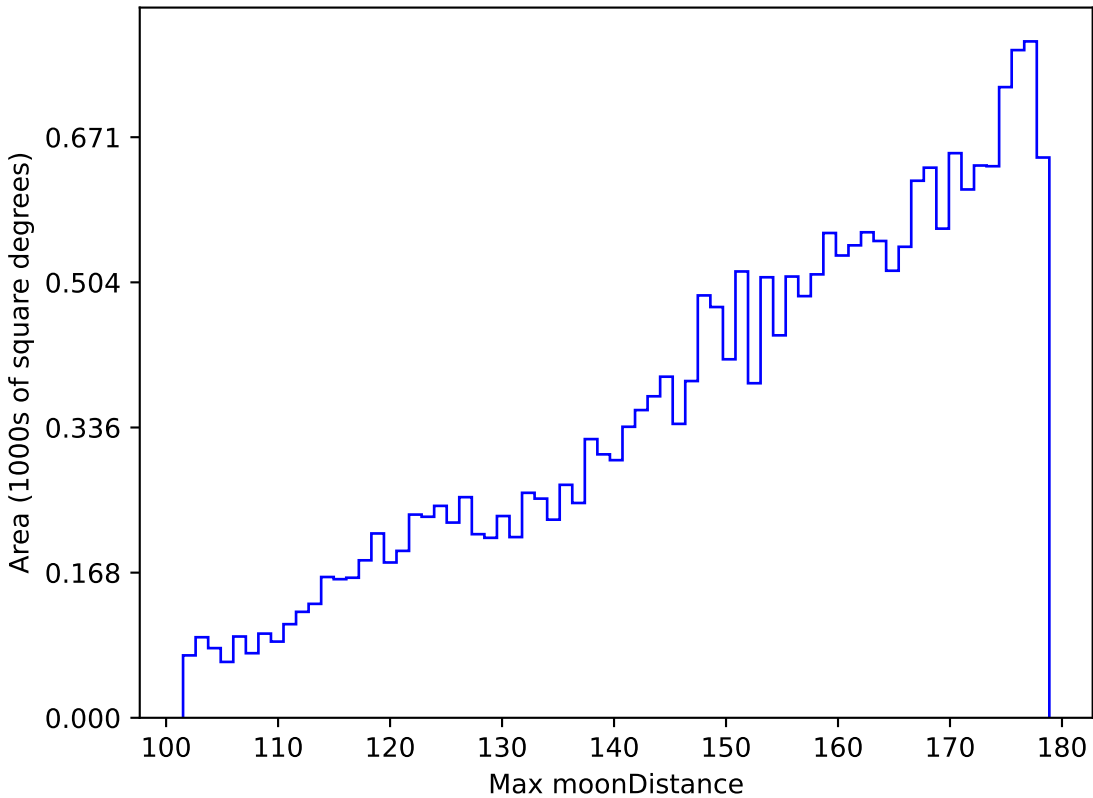
too_elab_r64_d3_giz_v3.4_10yrs All sky u band: Max moonDistance
