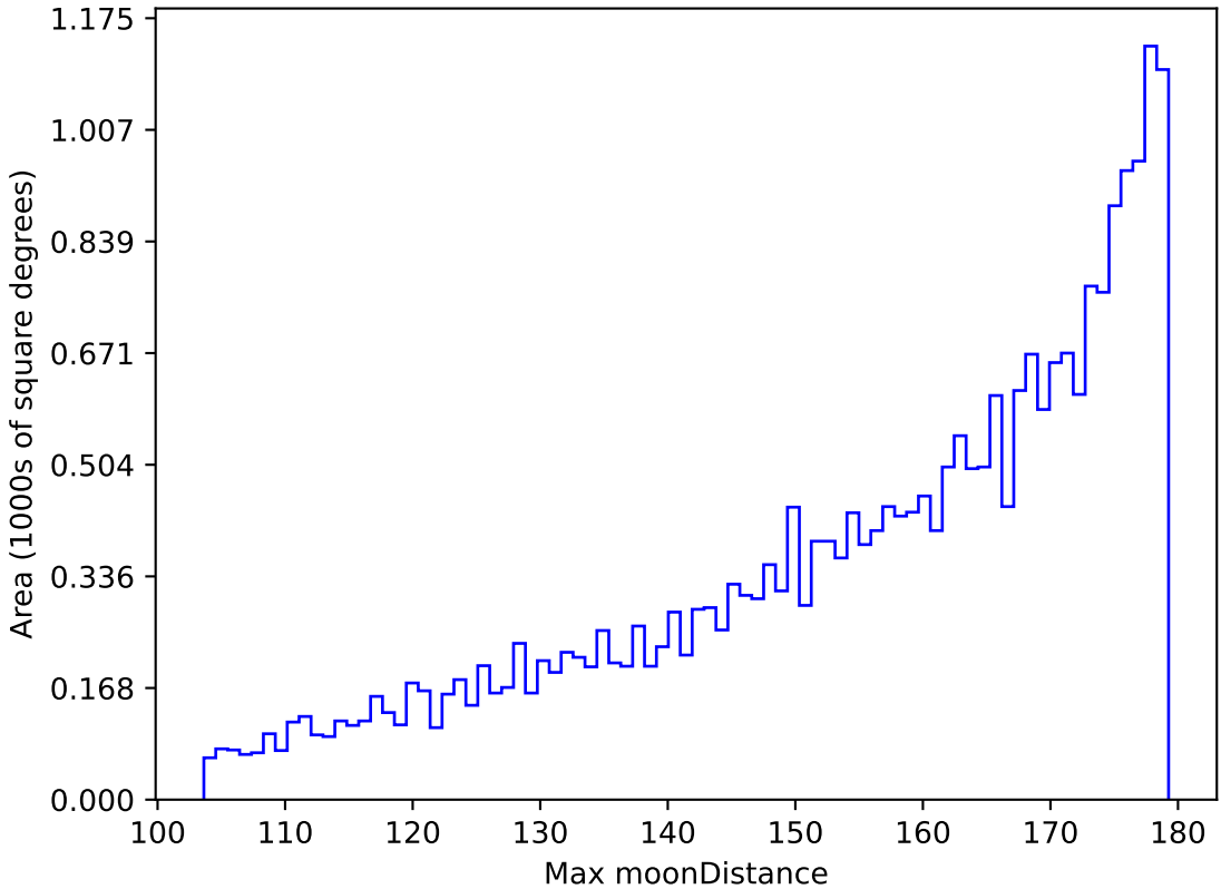
too_elab_r64_d3_giz_v3.4_10yrs All sky r band: Max moonDistance
