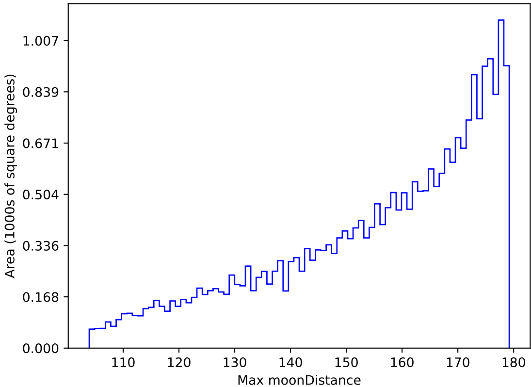
too_elab_r64_d3_giz_v3.4_10yrs All sky i band: Max moonDistance
