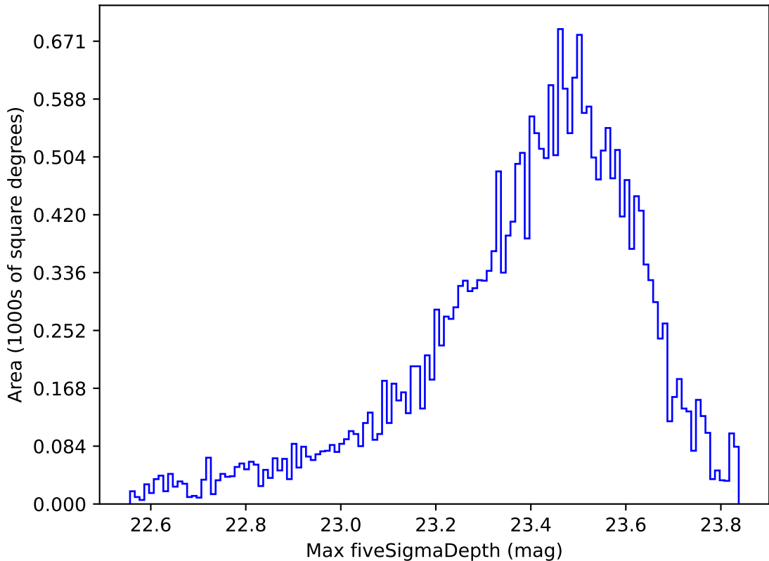
too_elab_r64_d3_giz_v3.4_10yrs Yr 1 z band: Max fiveSigmaDepth
