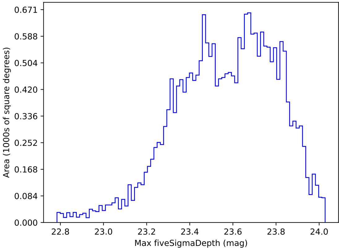
too_elab_r64_d3_giz_v3.4_10yrs Yr 1 u band: Max fiveSigmaDepth
