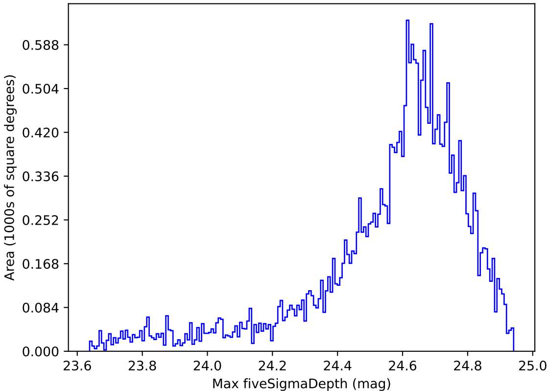
too_elab_r64_d3_giz_v3.4_10yrs Yr 1 r band: Max fiveSigmaDepth
