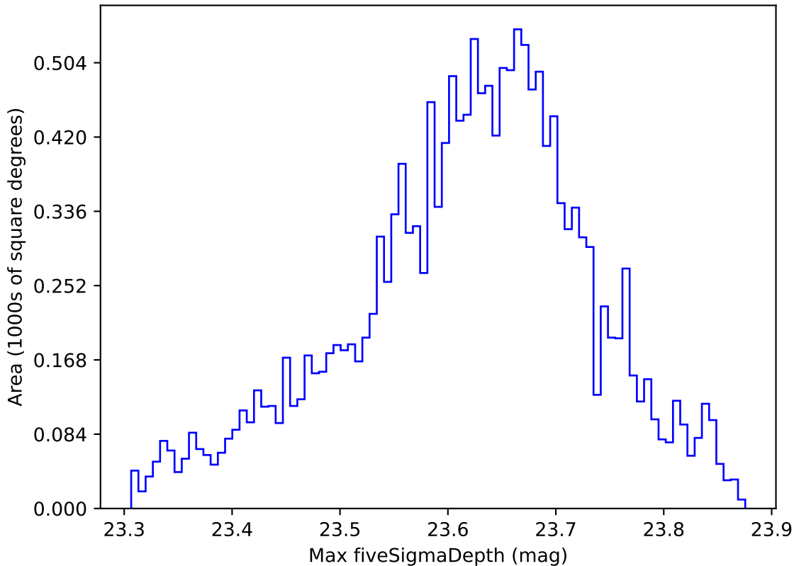
too_elab_r64_d3_giz_v3.4_10yrs WFD z band: Max fiveSigmaDepth
