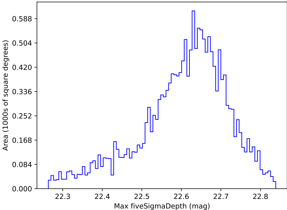
too_elab_r64_d3_giz_v3.4_10yrs WFD y band: Max fiveSigmaDepth
