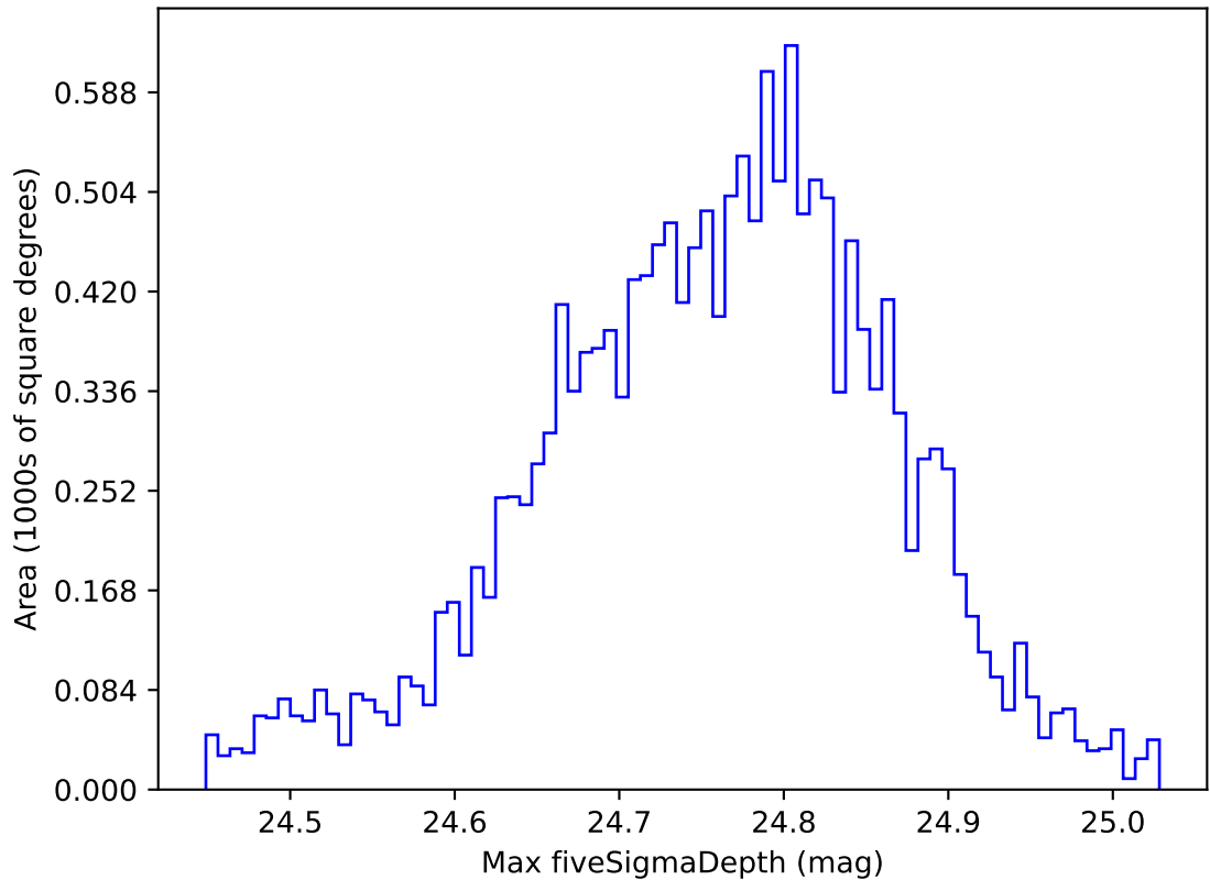
too_elab_r64_d3_giz_v3.4_10yrs WFD r band: Max fiveSigmaDepth
