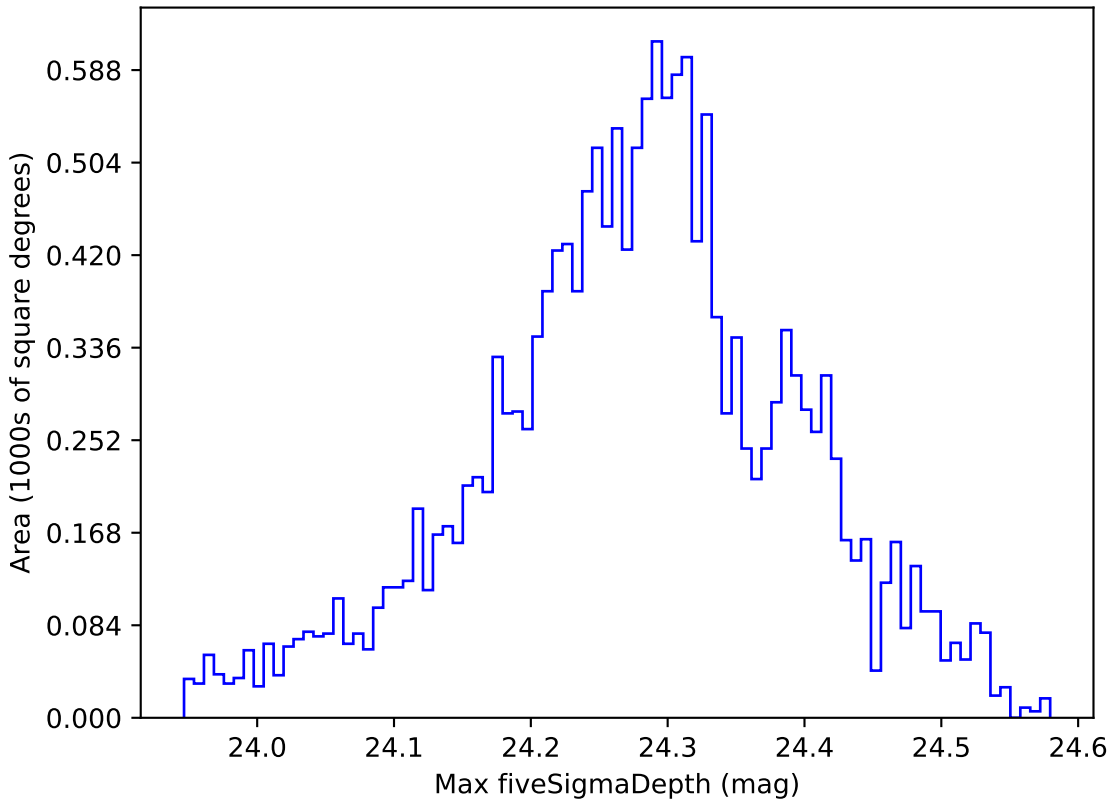
too_elab_r64_d3_giz_v3.4_10yrs WFD i band: Max fiveSigmaDepth
