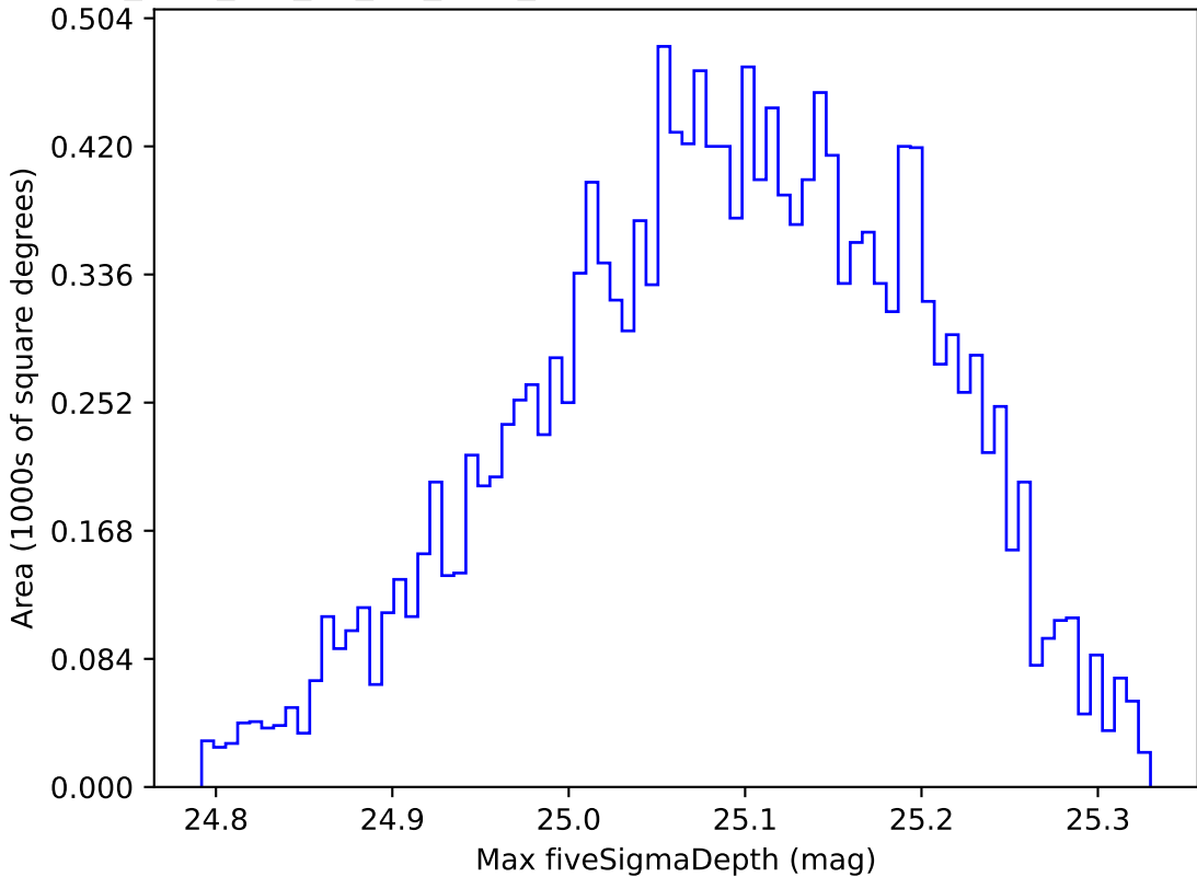
too_elab_r64_d3_giz_v3.4_10yrs WFD all bands: Max fiveSigmaDepth
