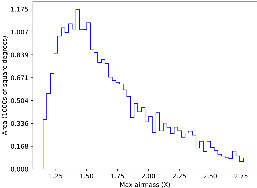
too_elab_r64_d3_giz_v3.4_10yrs Yr 1 z band: Max airmass
