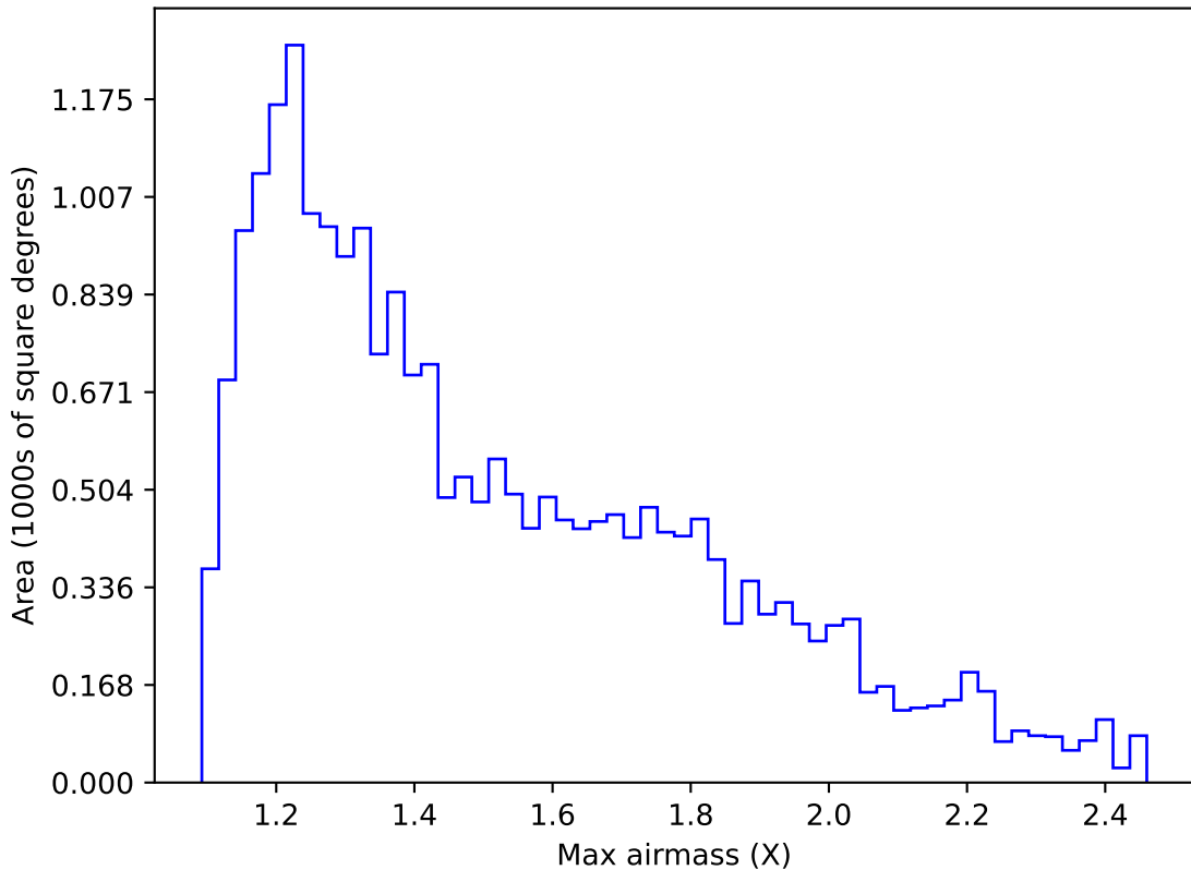
too_elab_r64_d3_giz_v3.4_10yrs Yr 1 u band: Max airmass
