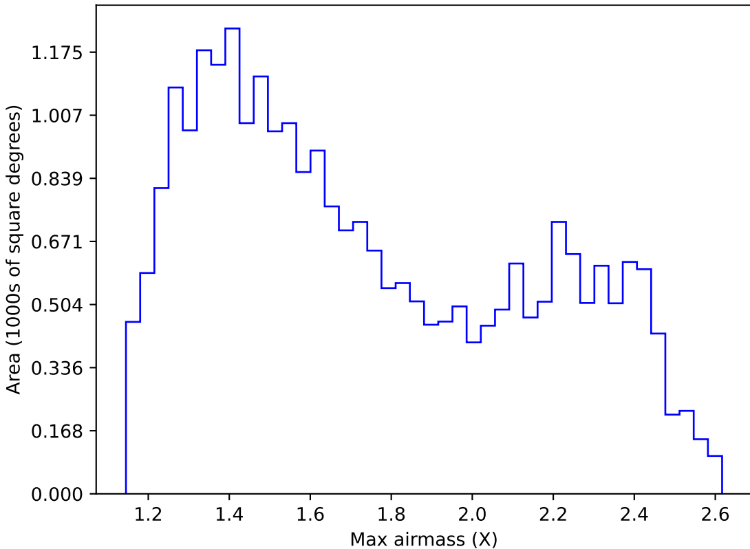
too_elab_r64_d3_giz_v3.4_10yrs Yr 1 r band: Max airmass
