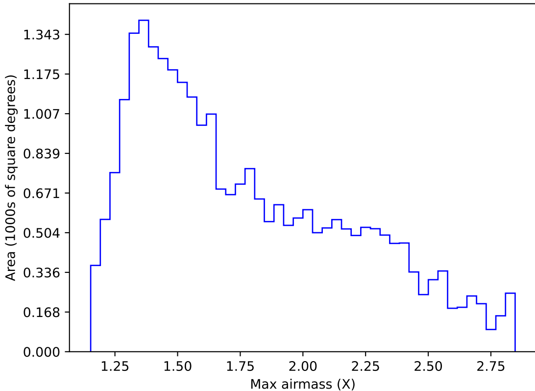
too_elab_r64_d3_giz_v3.4_10yrs Yr 1 i band: Max airmass
