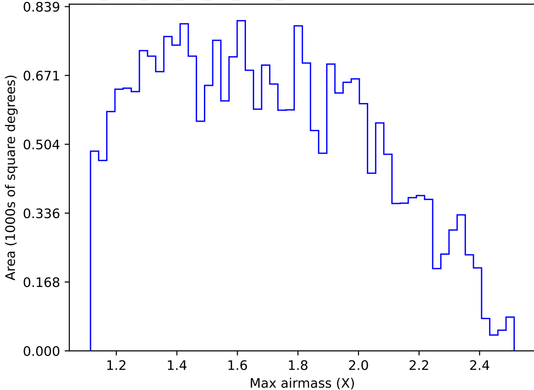
too_elab_r64_d3_giz_v3.4_10yrs Yr 1 g band: Max airmass
