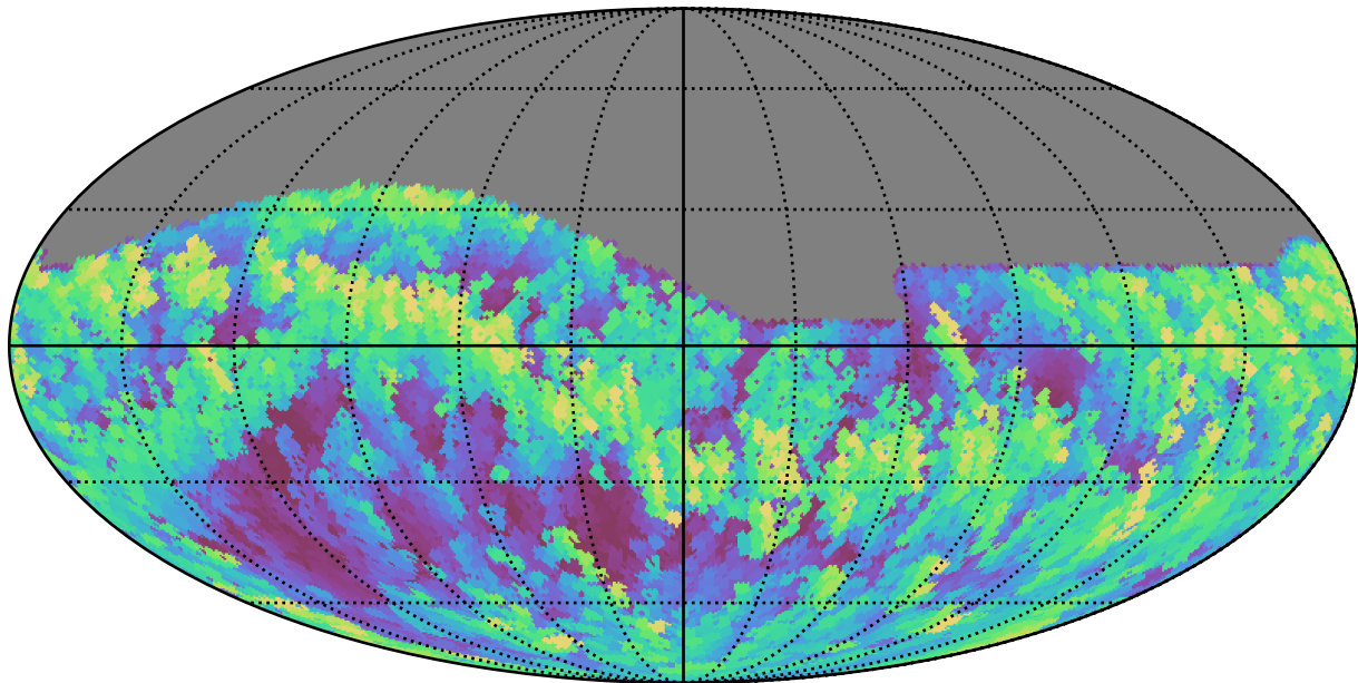
too_elab_r64_d3_giz_v3.4_10yrs Yr 1 all bands: Max airmass
