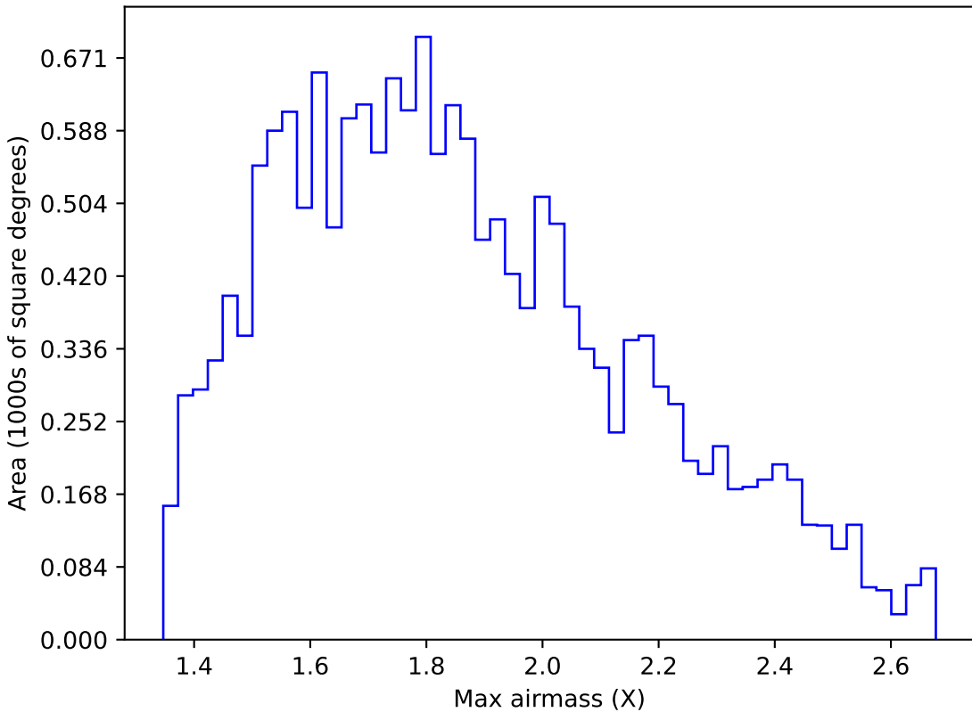
too_elab_r64_d3_giz_v3.4_10yrs WFD u band: Max airmass
