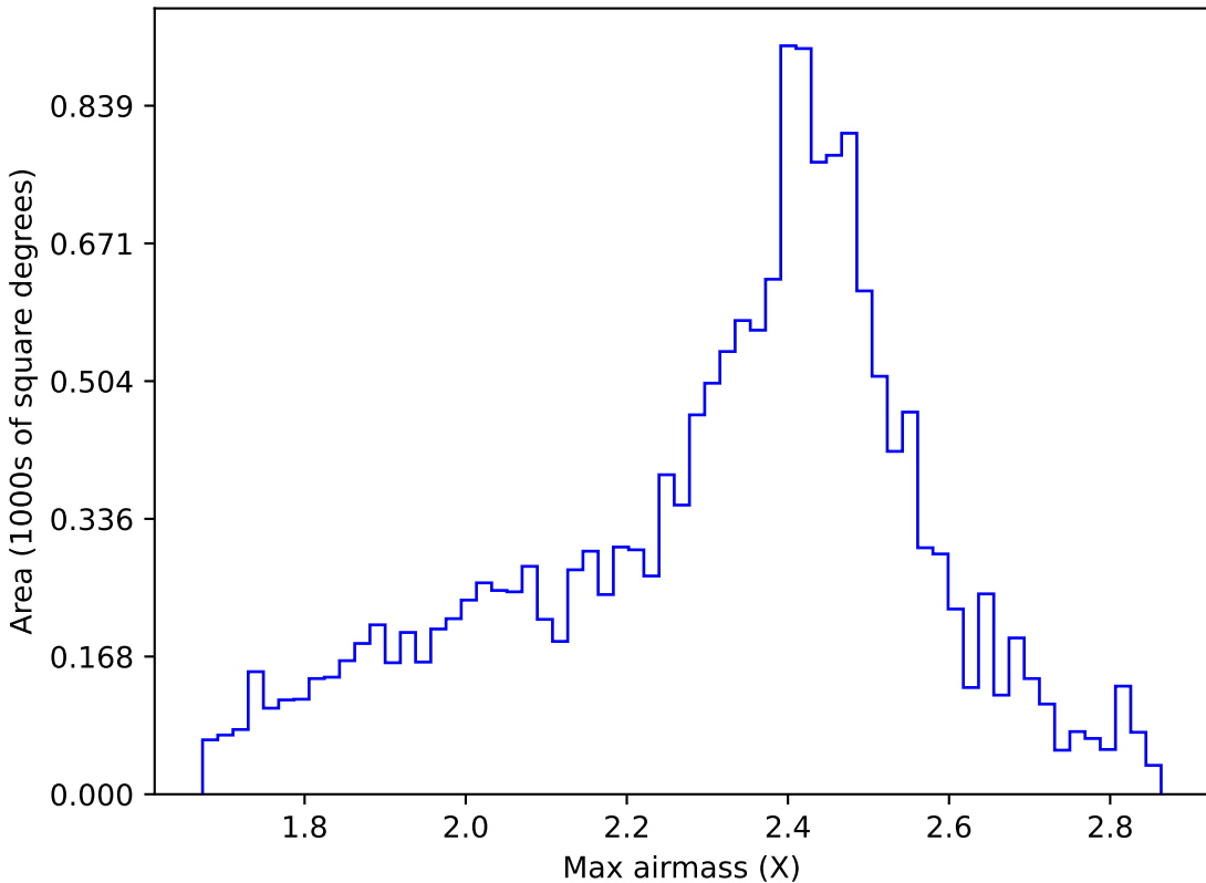
too_elab_r64_d3_giz_v3.4_10yrs WFD r band: Max airmass
