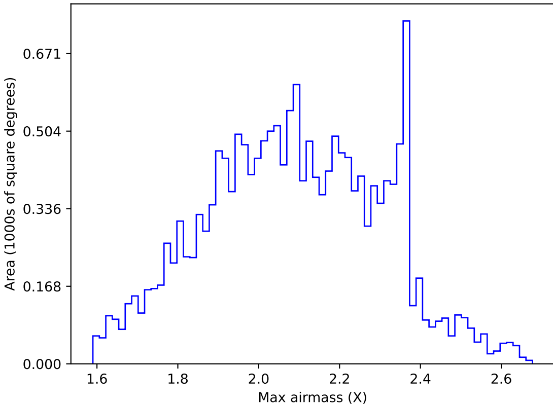
too_elab_r64_d3_giz_v3.4_10yrs WFD g band: Max airmass
