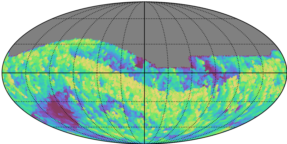
too_elab_r64_d3_giz_v3.4_10yrs All sky z band: Max airmass
