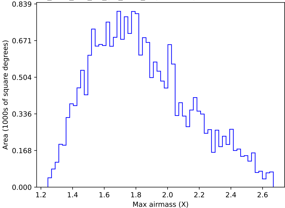
too_elab_r64_d3_giz_v3.4_10yrs All sky u band: Max airmass
